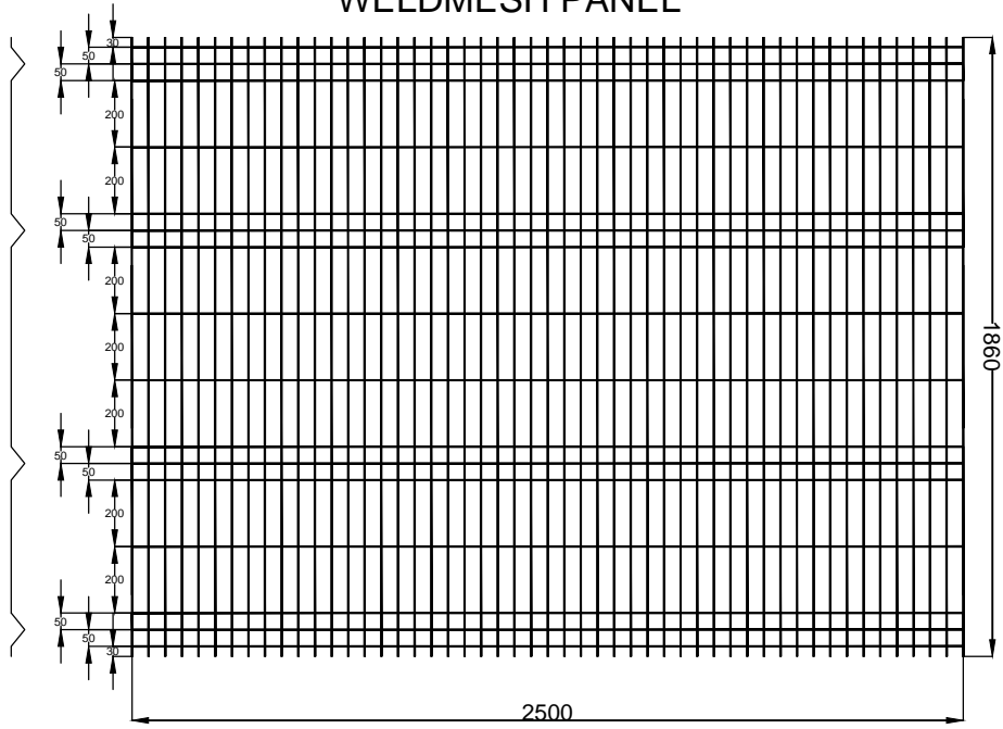
FRONT VIEW - WITH BEND
