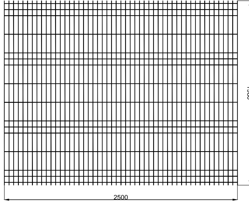
FRONT VIEW - W/O BEND
